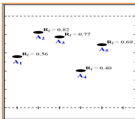
Figure 11. TLC spots and R f of [A 1 -A 5 ]
