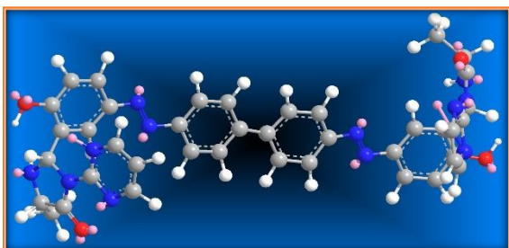
Figure 8. Stereochemistry of [A 3 ]
