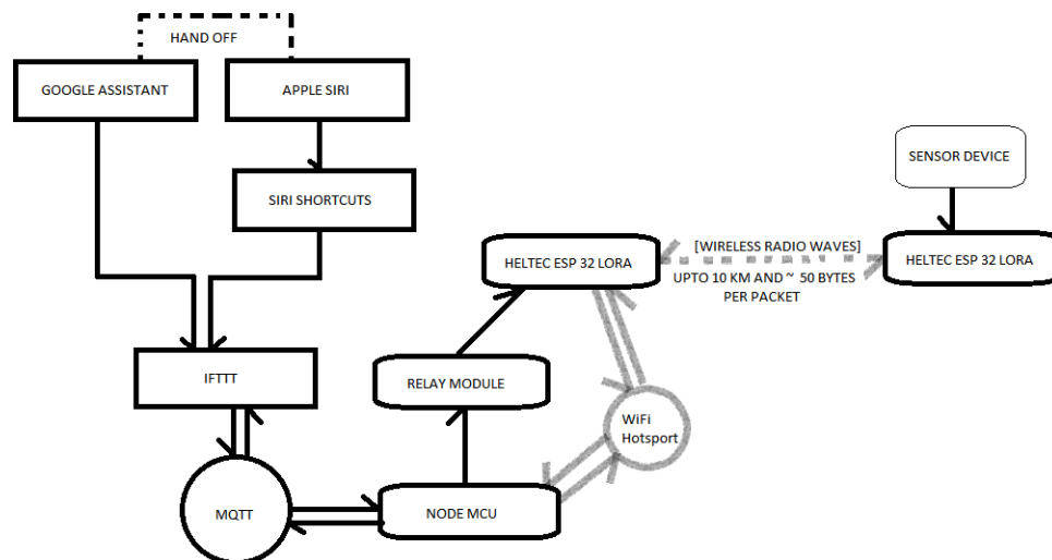
Fig 1. Architecture Design of the Complete System
