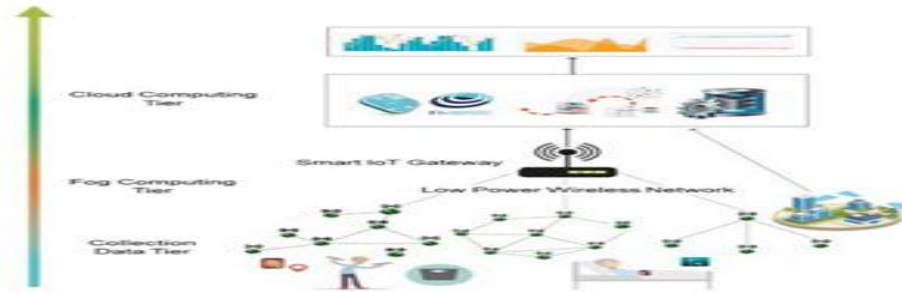
Fig 1. High-level view of the hierarchical proposed architecture.
