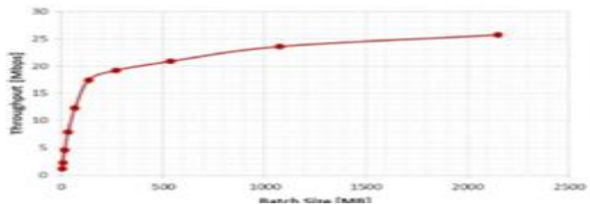
Fig 8. Big Data Analyzer performance
