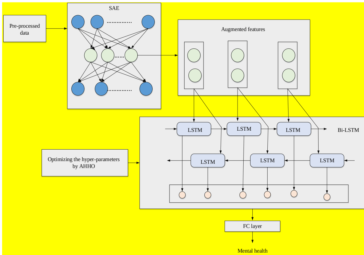
Figure 3. Architecture of SAE-O-Bi-LSTM
