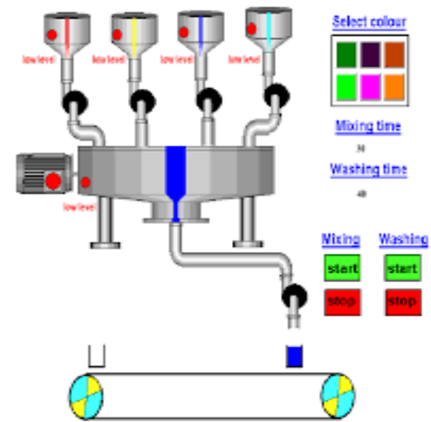
Fig 3. SCADA representation of paint mixing machine using the same recipe making concept
